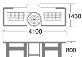
CM.040 ROULETTE TABLE DETACHABLE TYPE (DOUBLE)
